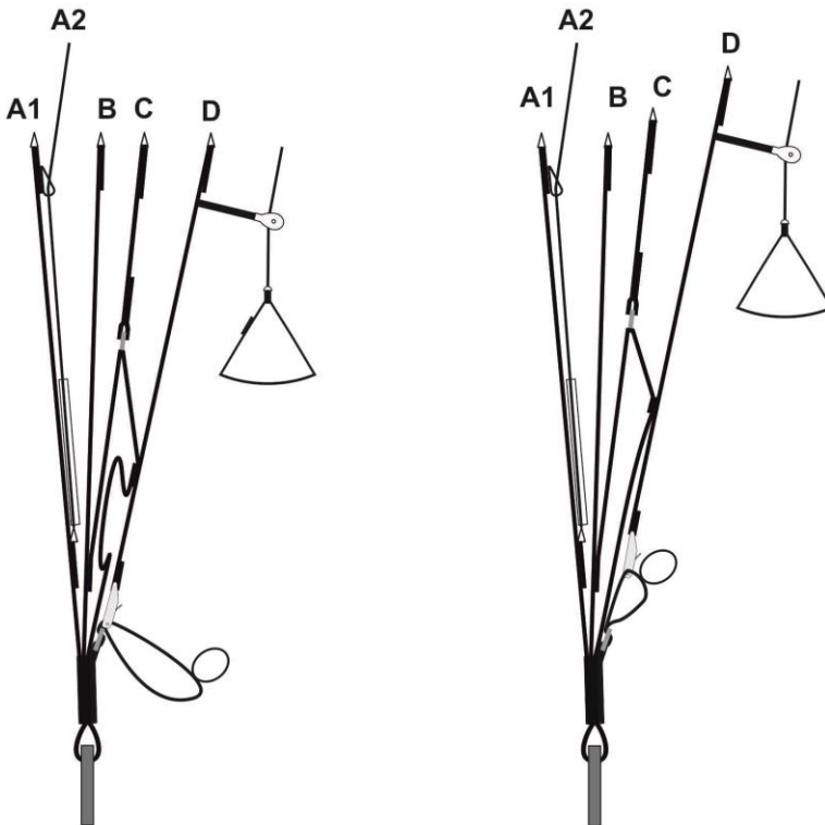
Fig. 6: TWIN 5 risers showing how the trimmers work
